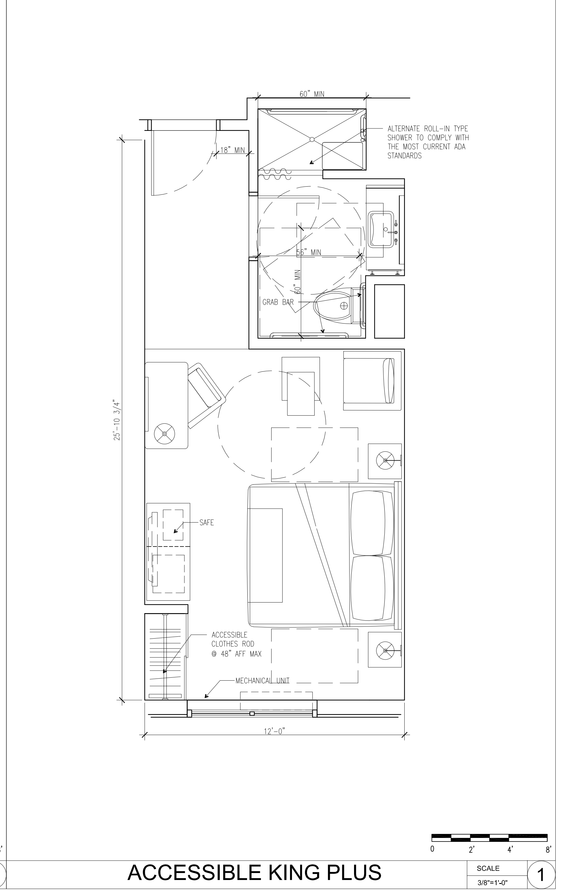
ACCESSIBLE ROOM CONFIGURATION
